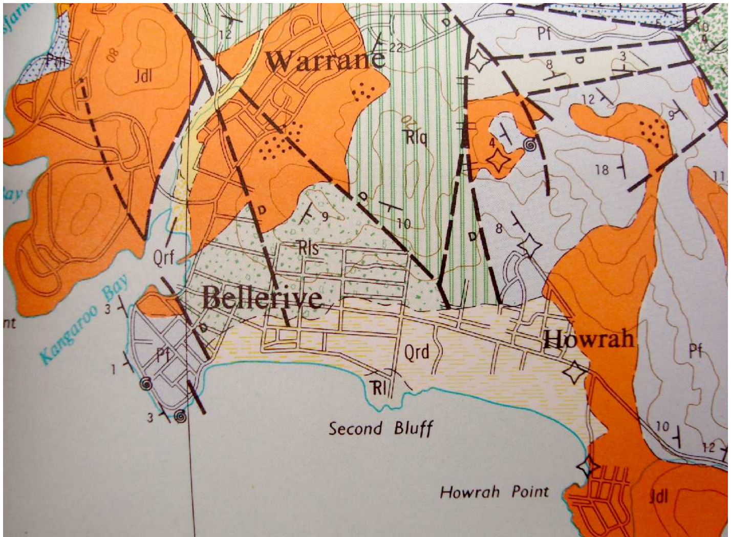
From: Geological Atlas 1:50,000 Map Series - HOBART 1973 Bellerive & Howrah Basins
